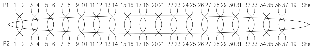
Pin assignment
