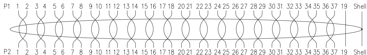
Pin assignment
