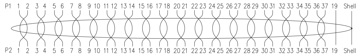
Pin assignment
