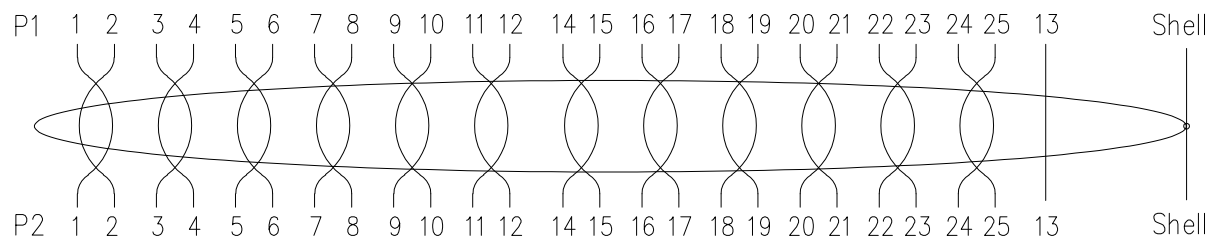
Pin assignment
