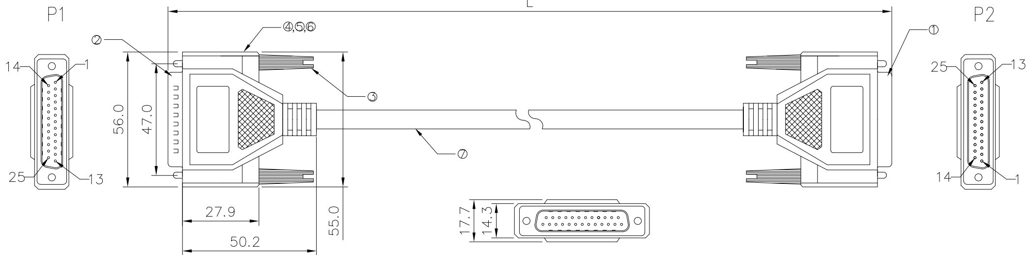
Pin assignment
