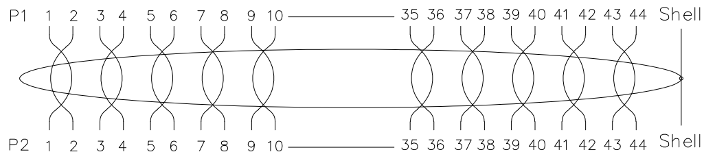
Pin assignment
