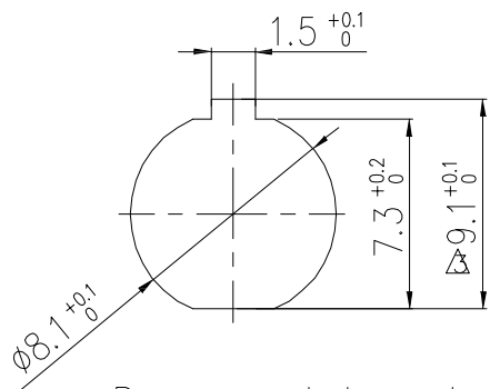
Recommended panel size
