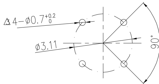
Recommended PCB size
