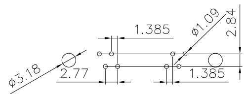
PCB layout
