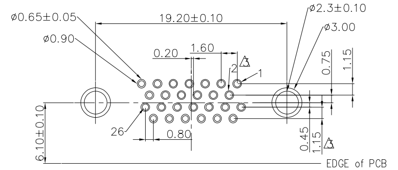
PCB layout
