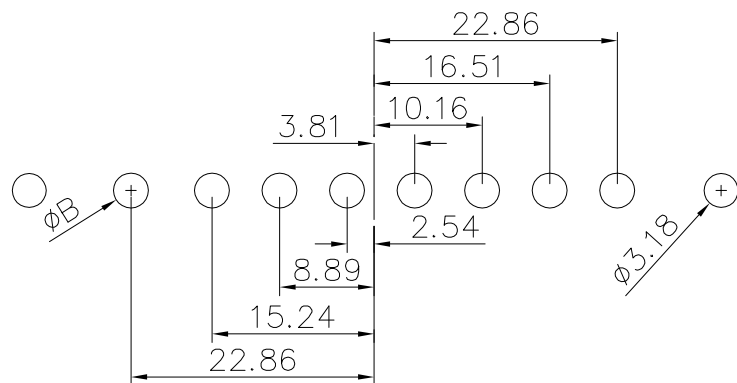
PCB layout
