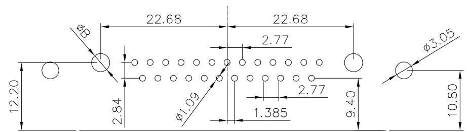
PCB layout
