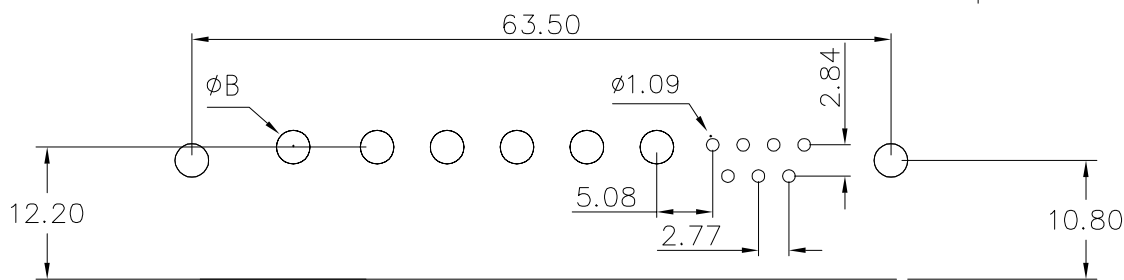
PCB layout
