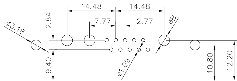
PCB layout
