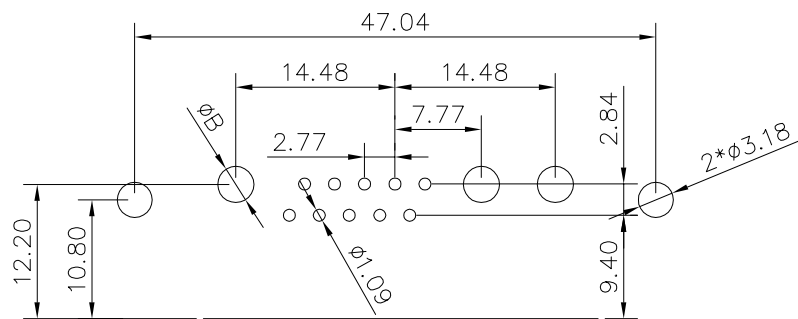
PCB layout
