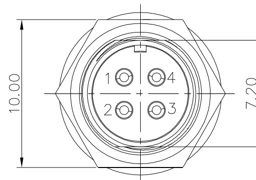
Soldering face
