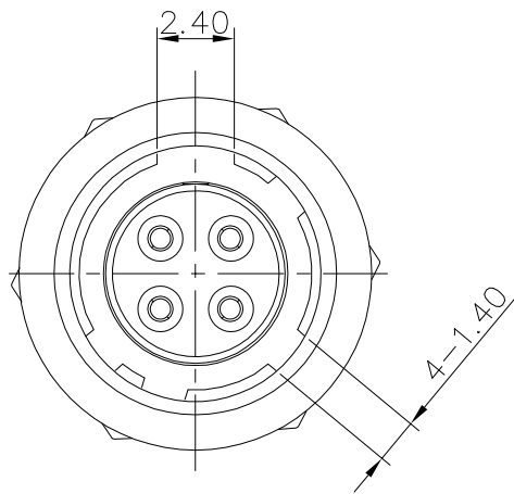
Mating face
