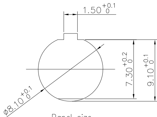
Panel size
