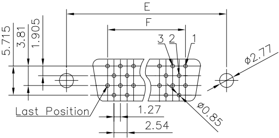
PCB Layout (14,26,50 Pos)
