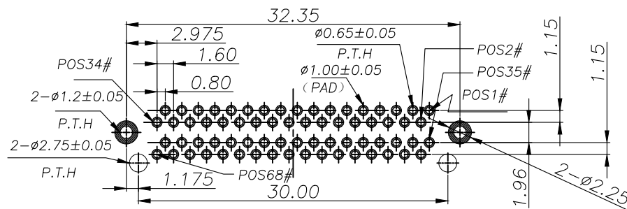
Recommended P.C.B Layout T=1.6MM
