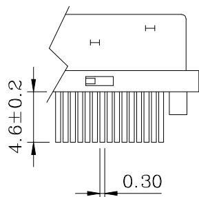
Detail A Scale 1.5:1
