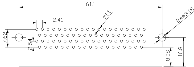
PCB Layout
