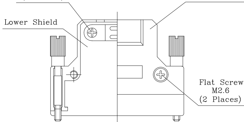
Flat Screw M2.6 (2 Places)
