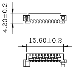
Wire Holder (2 Places)
