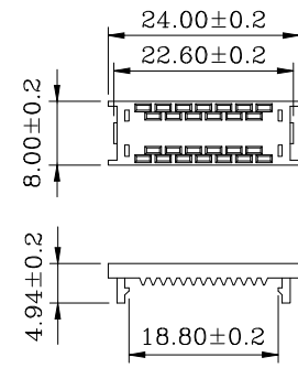
Termination Cover (1 Places)
