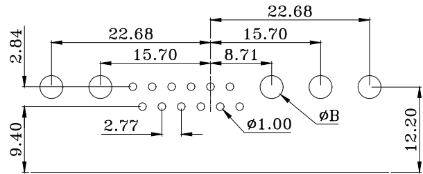
PCB LAYOUT
